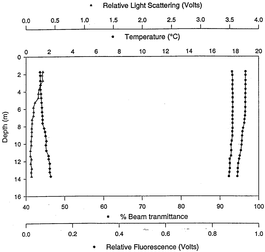
Figure A.29b - Station 4.2 Downcast
