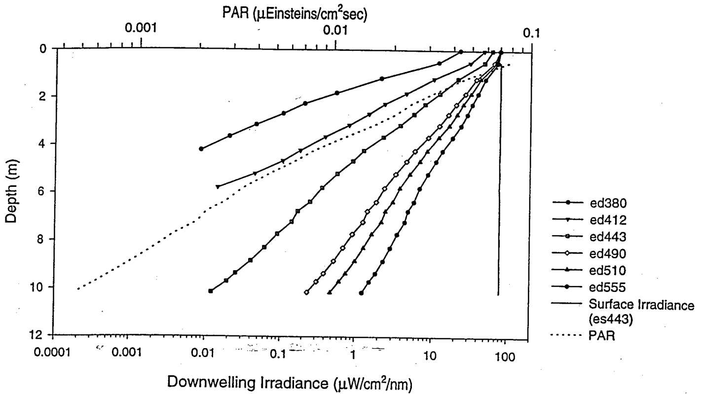
Figure A.4a - Station 1.2 Upcast
