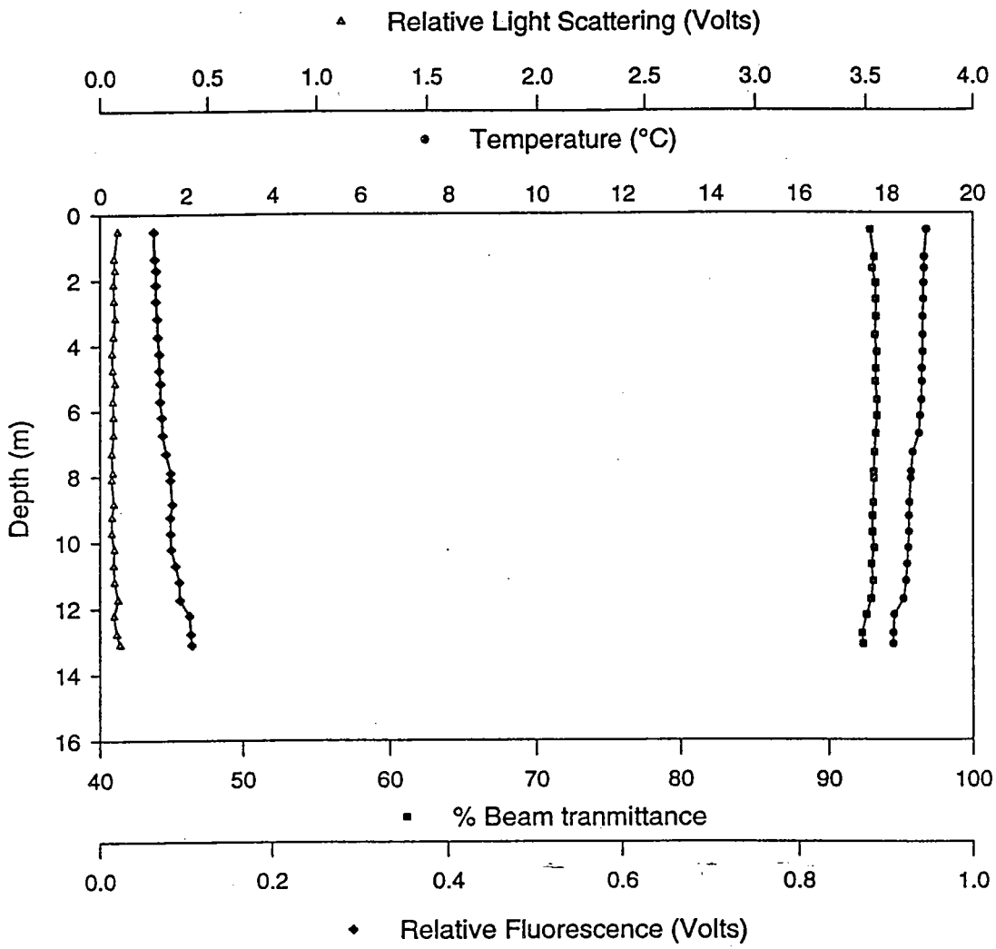
Figure A.30b - Station 4.2 Upcast
