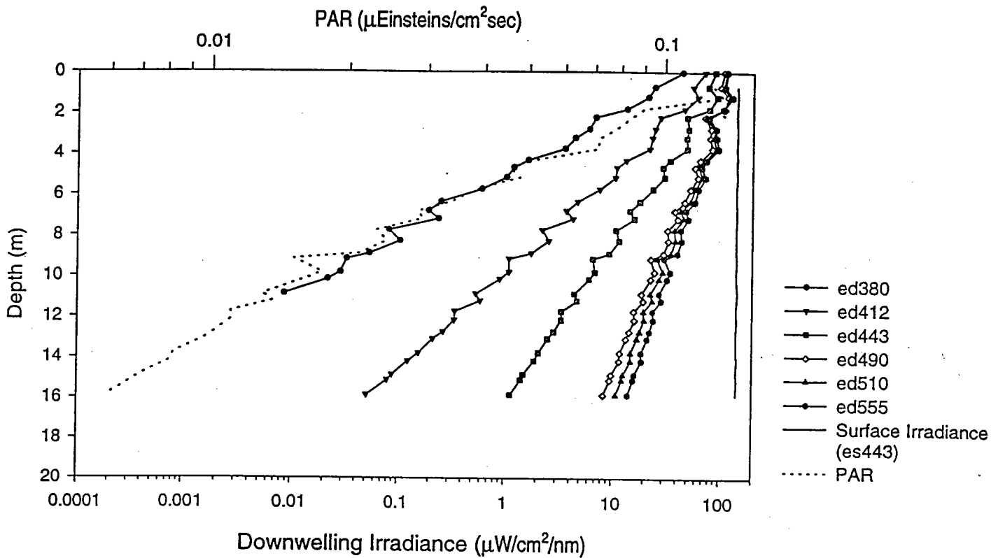
Figure A.24a - Station 3.2 Upcast
