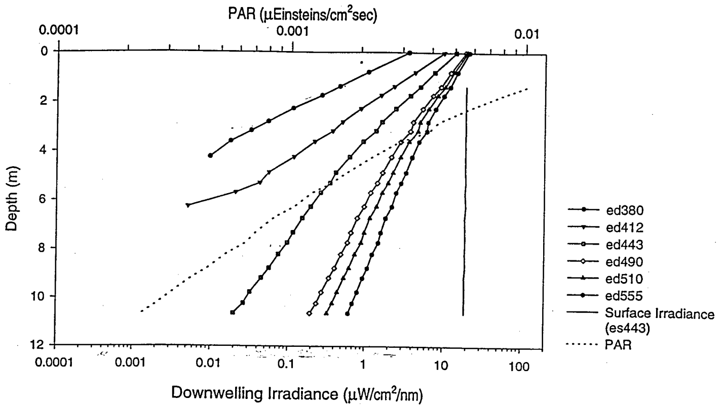
Figure A.5a - Station 1.3 Downcast
