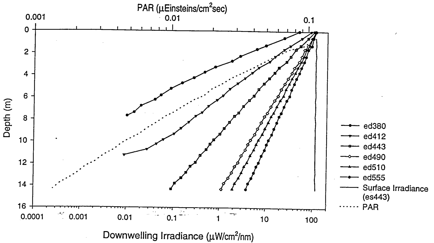
Figure A.2a - Station 1.1 Upcast
