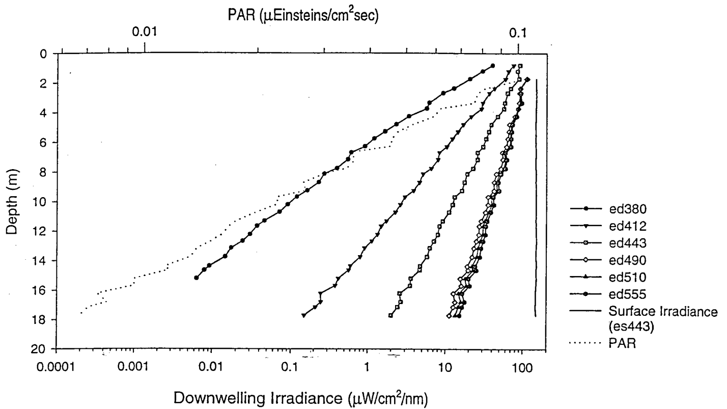
Figure A.15a - Station 2.5 Downcast
