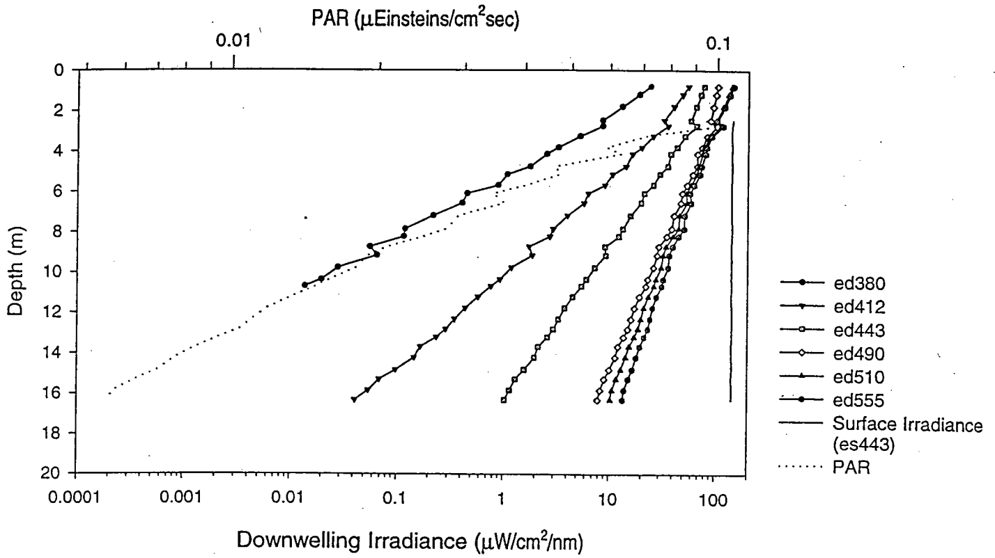
Figure A.23a - Station 3.2 Downcast
