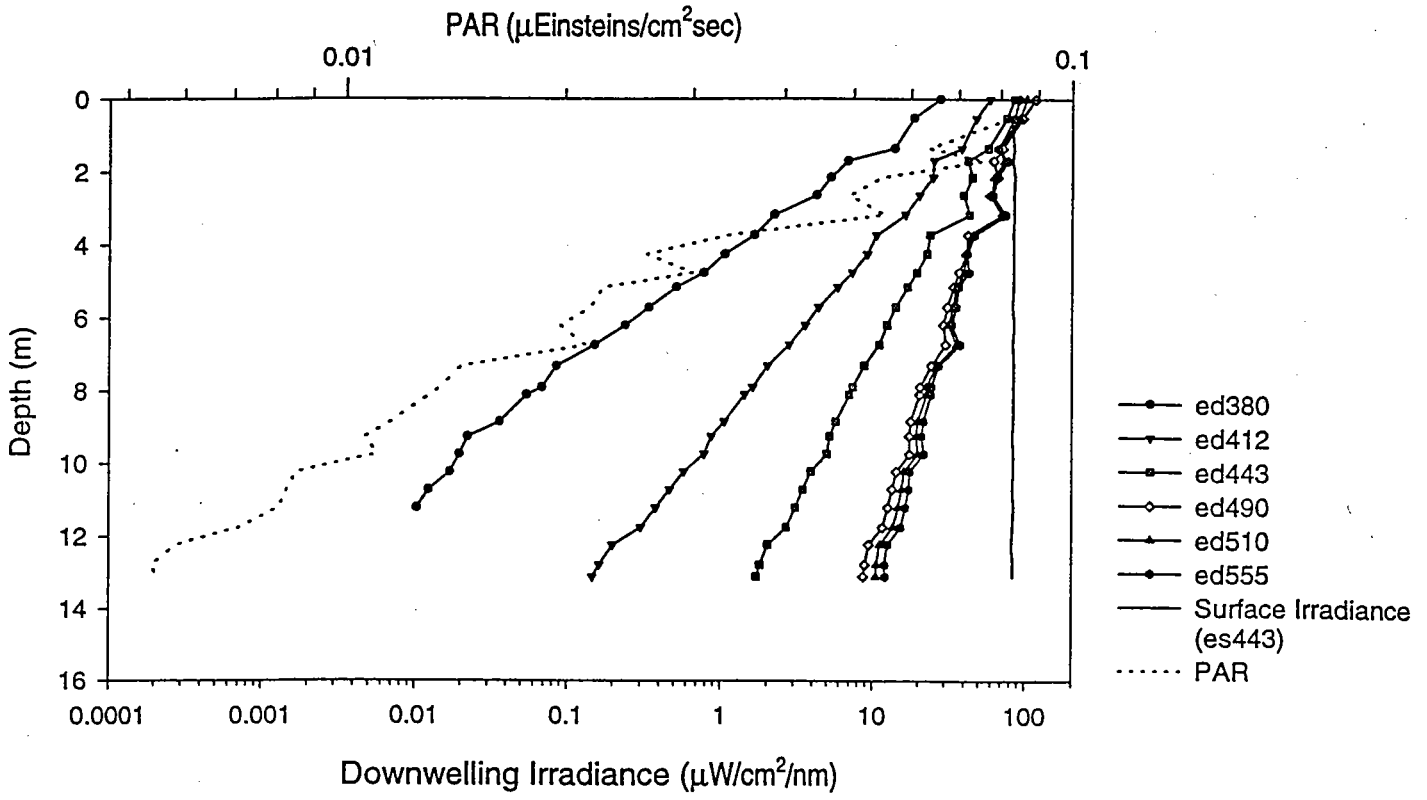
Figure A.30a - Station 4.2 Upcast
