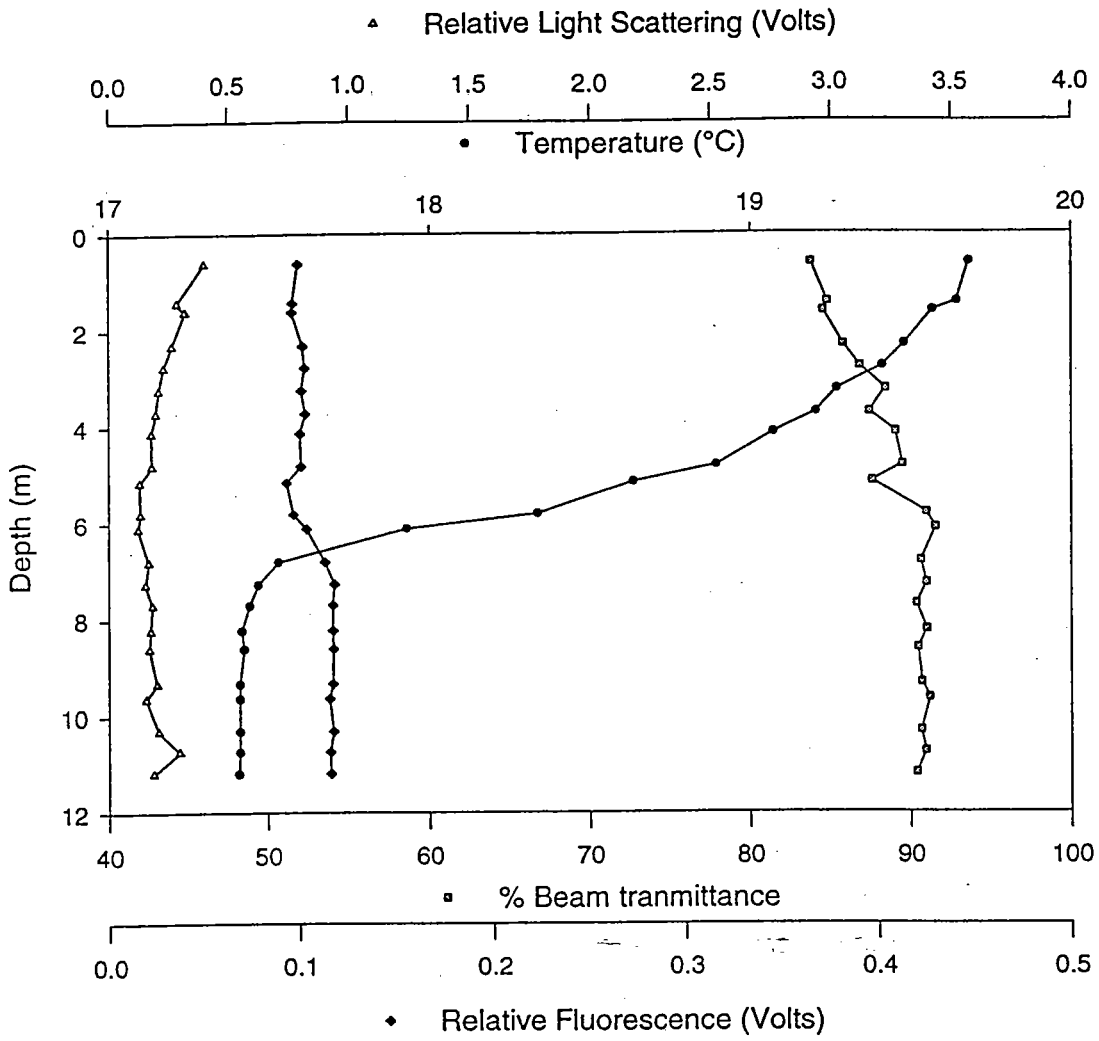
Figure A.12b - Station 2.3 Upcast
