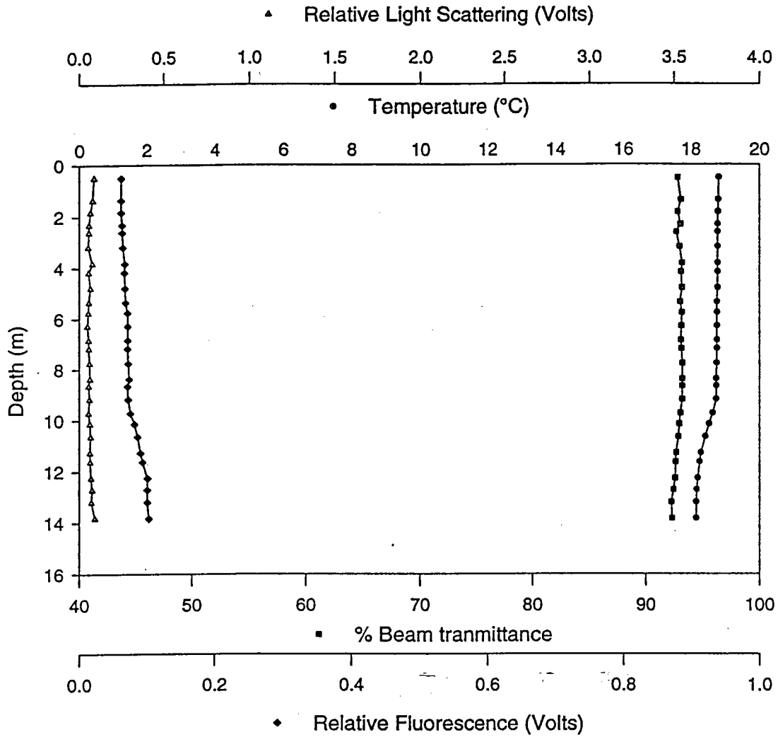
Figure A.28b - Station 4.1 Upcast
