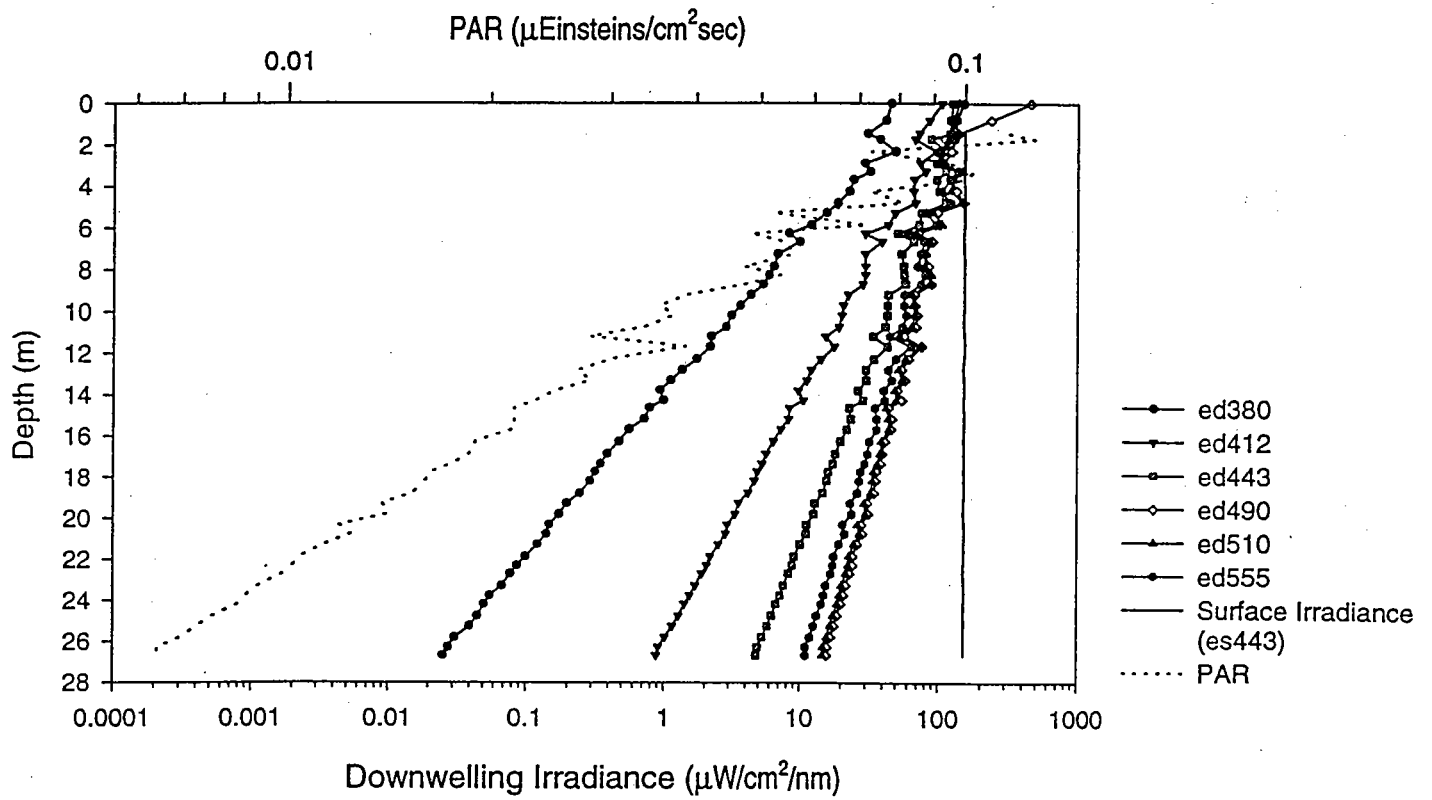
Figure A.31a - Station 4.3 Downcast (W27)
