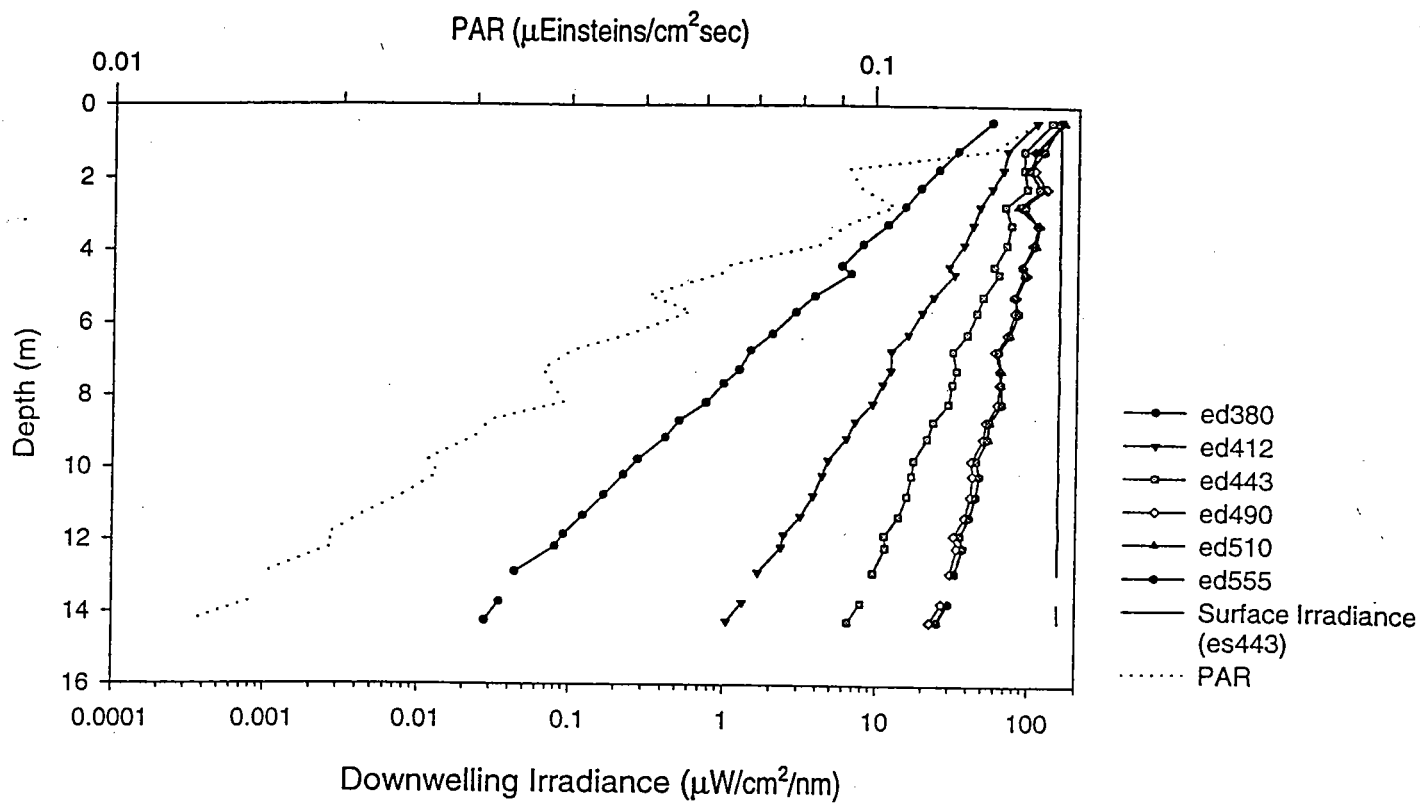
Figure A.26a - Station 3.3 Upcast
