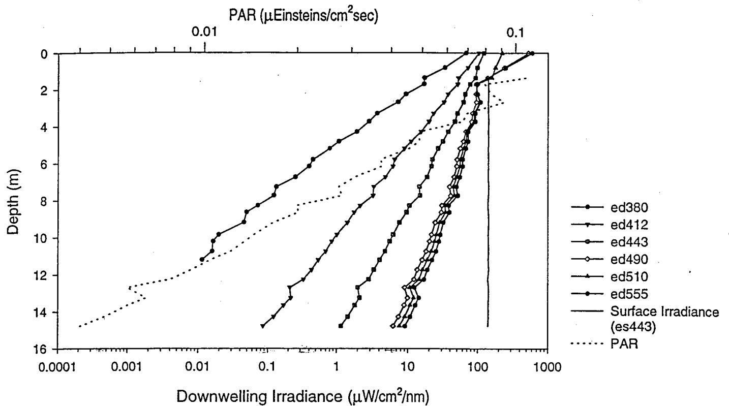
Figure A.13a - Station 2.4 Downcast
