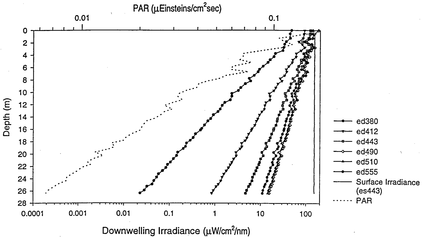
Figure A.32a - Station 4.3 Upcast
