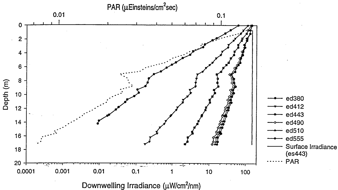
Figure A.16a - Station 2.5 Upcast
