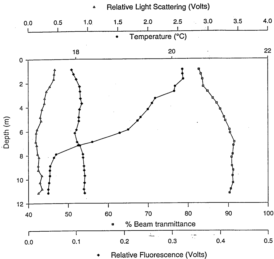
Figure A.11b - Station 2.3 Downcast
