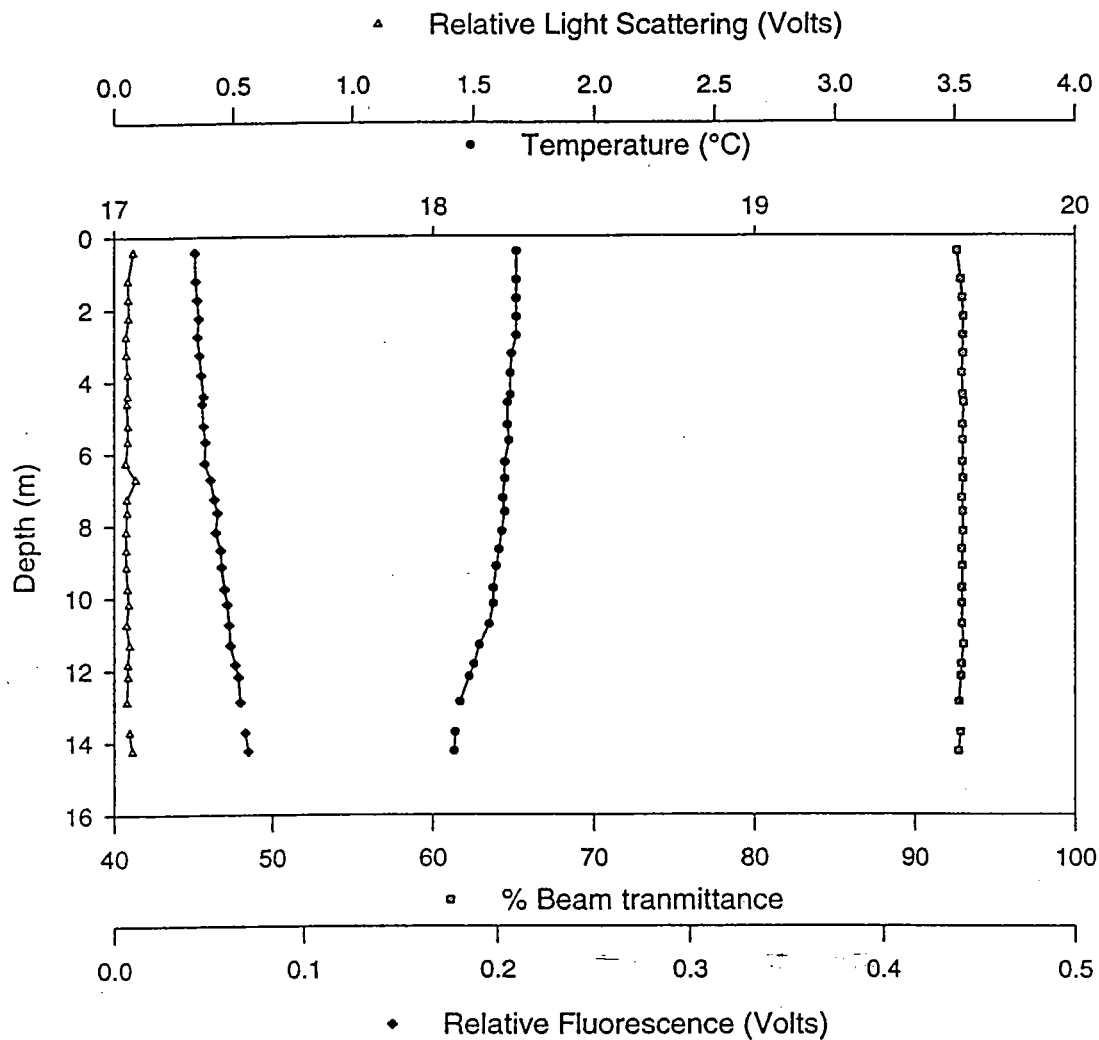
Figure A.26b - Station 3.3 Upcast
