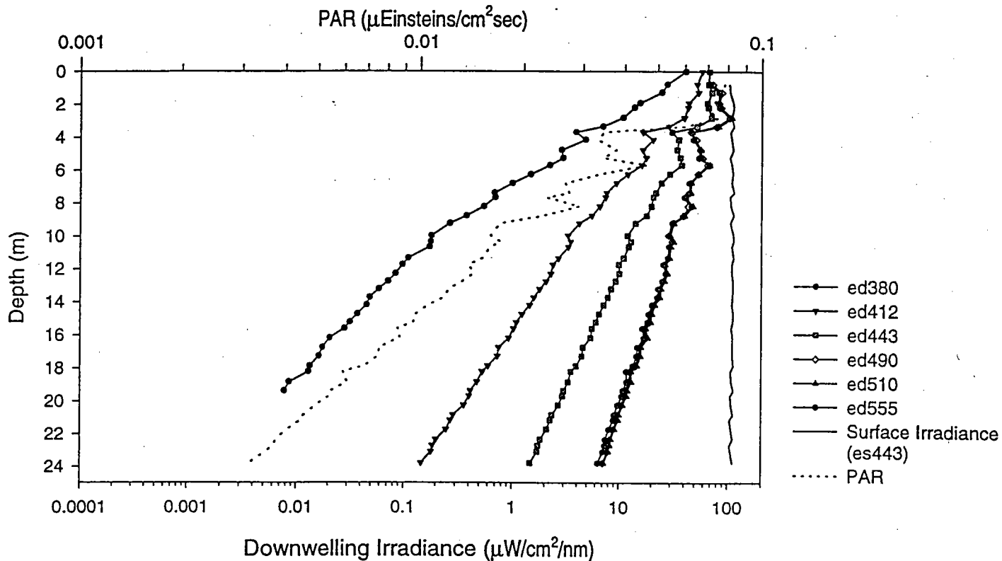
Figure A.19a - Station 2.7 Downcast
