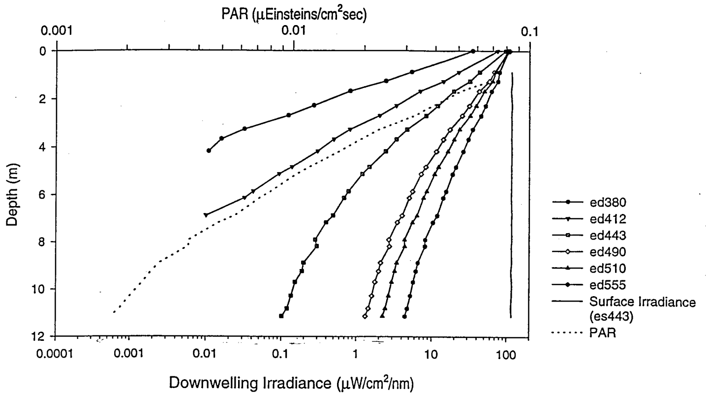
Figure A.11a - Station 2.3 Downcast
