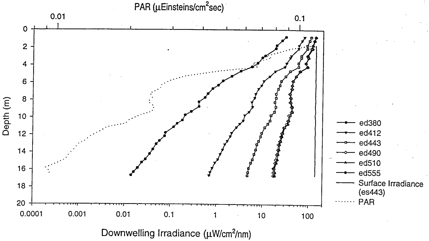
Figure A.17a - Station 2.6 Downcast
