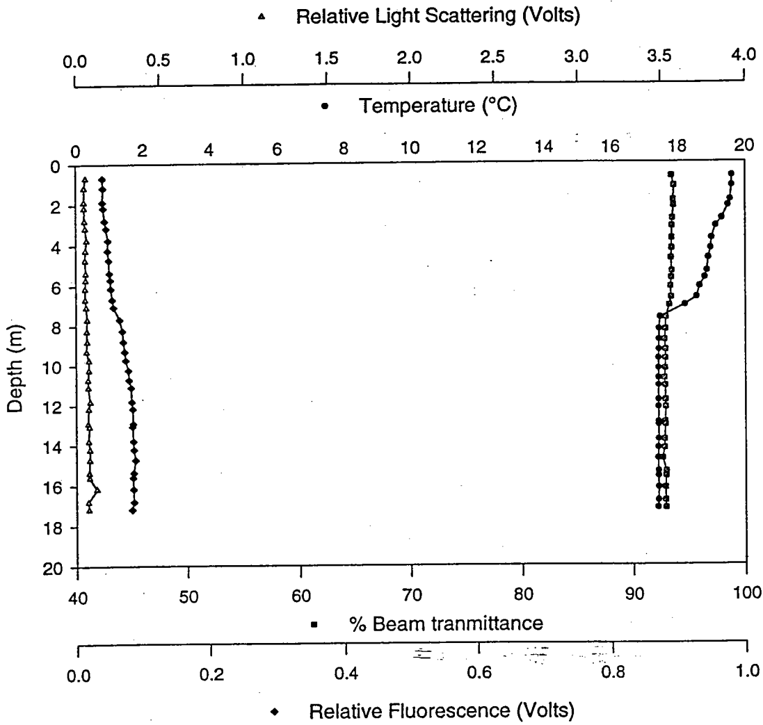
Figure A.16b - Station 2.5 Upcast
