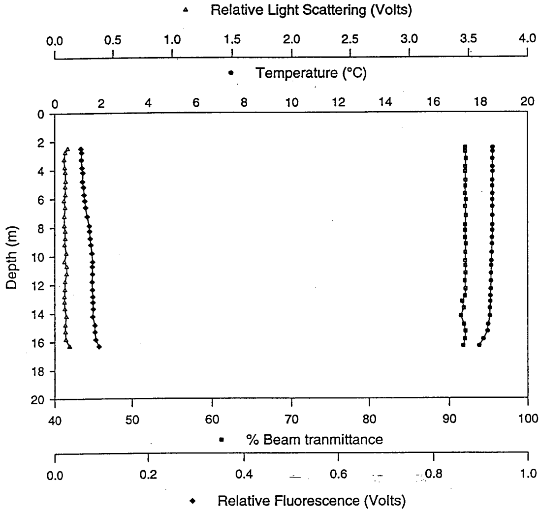
Figure A.23b - Station 3.2 Downcast
