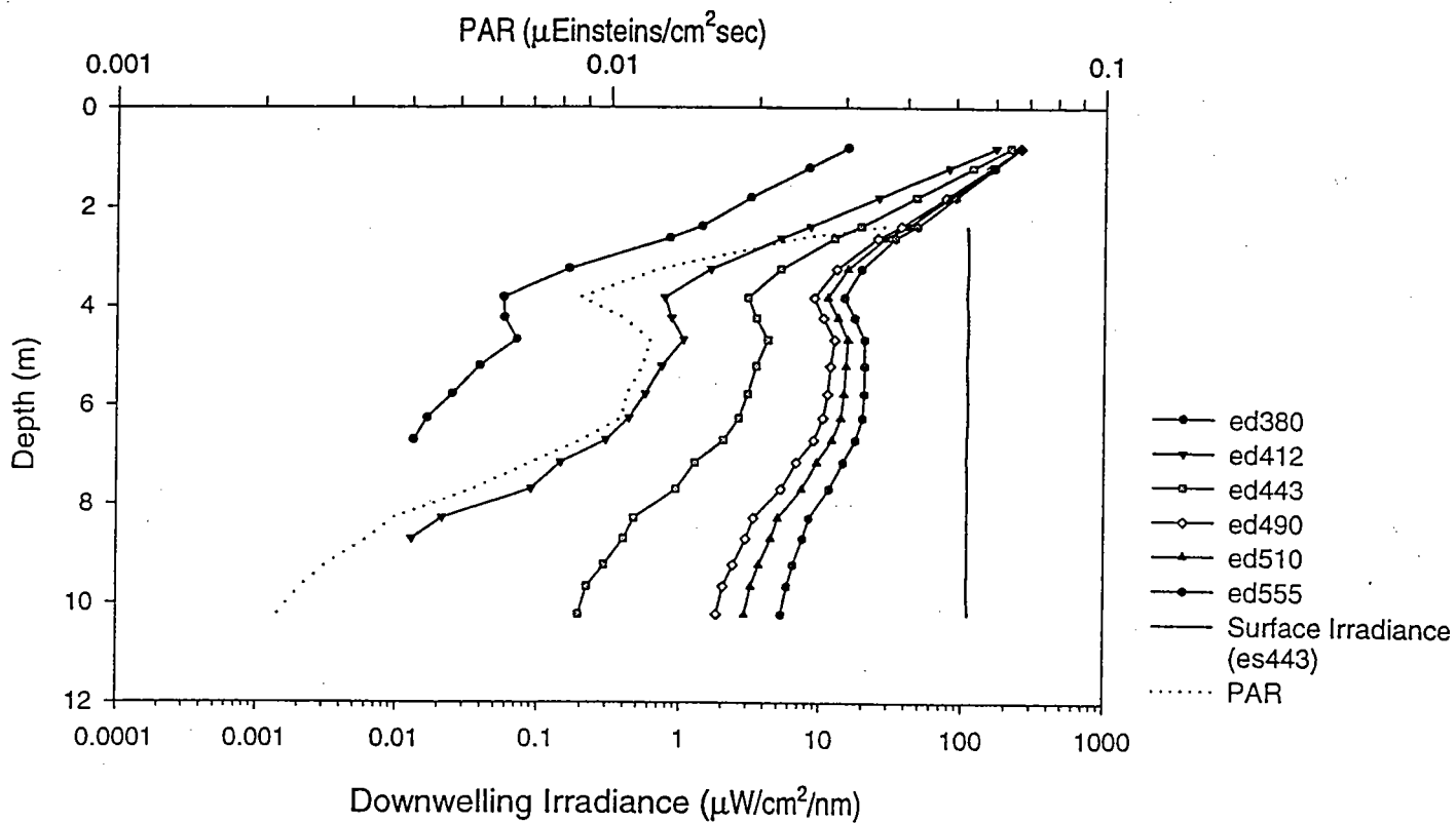
Figure A.21a - Station 3.1 Downcast
